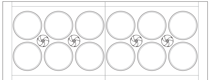
TOP VIEW 12+12
